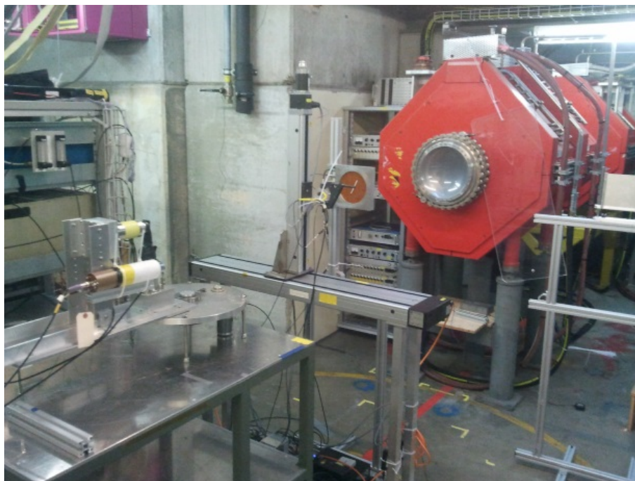
Figure 2. Experimental arrangement in the piM1 area.
