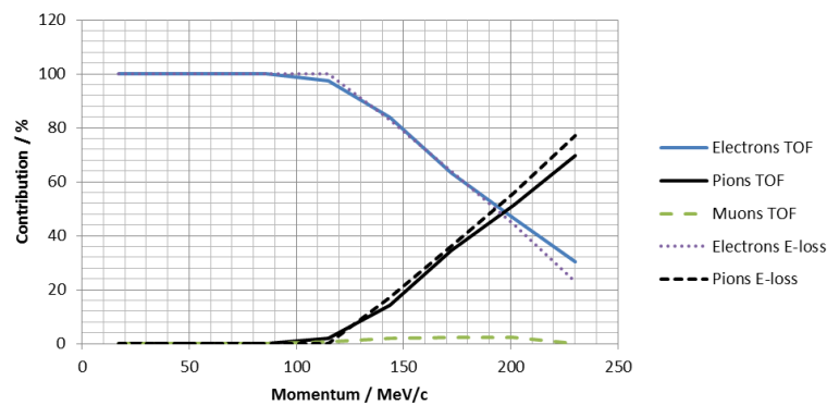
Figure 6. Relative contributions of electrons, muons and pions to the piM1 particle beams.
