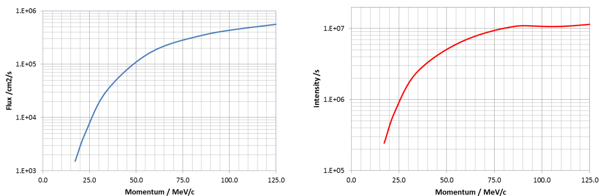
Figure 7. Maximum values of the electron flux and intensity for proton beam intensity of 2.1 mA.
