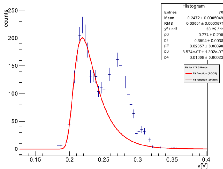
Figure 5. Spectrum of energy loss measured by the thick detector of the telescope at momentum 172 MeV/c.
