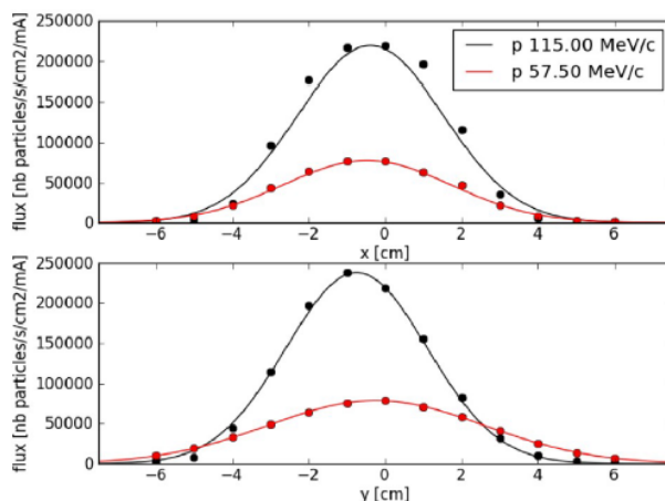
Figure 3. Example of electron beam profiles measured for two momentum values.
