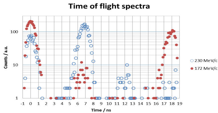
Figure 4. Time of flight spectra measured at two different momenta.
